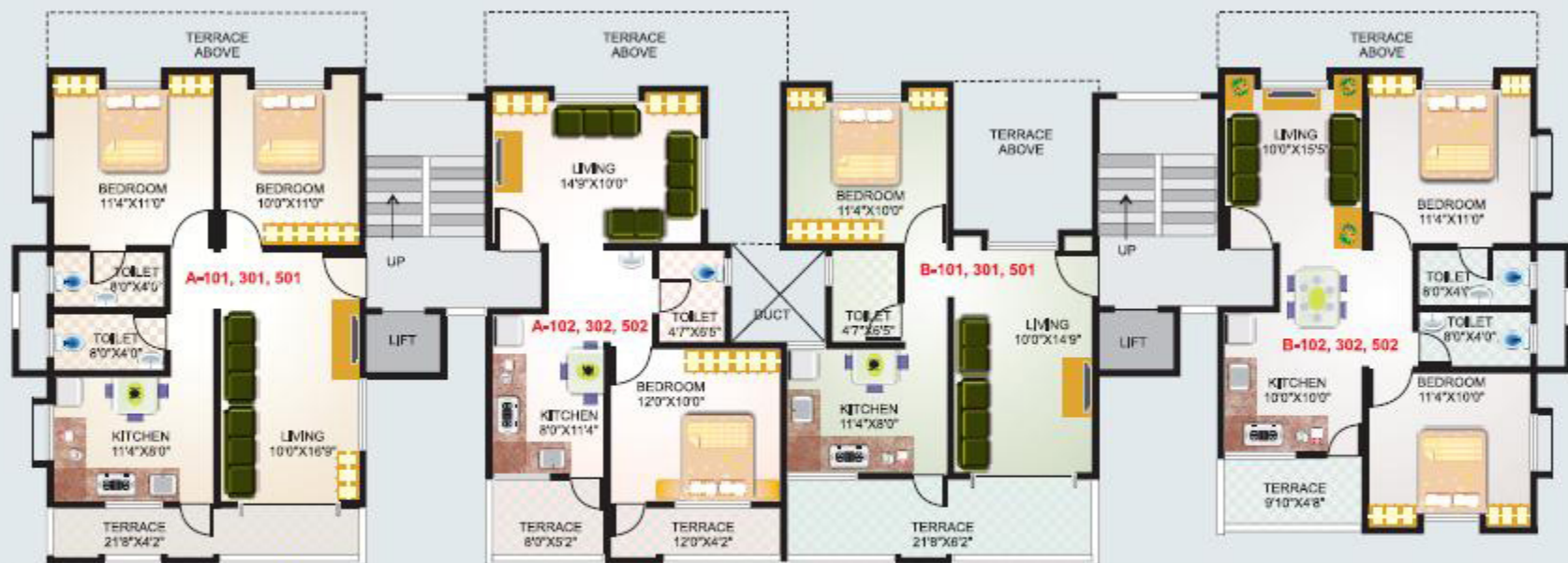
1st, 3rd & 5th Floor Plan
